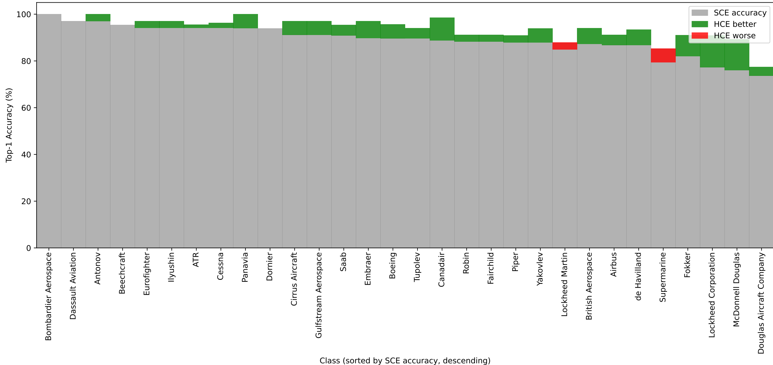
ResNet-50 — Per-manufacturer accuracy: SCE vs HCE
